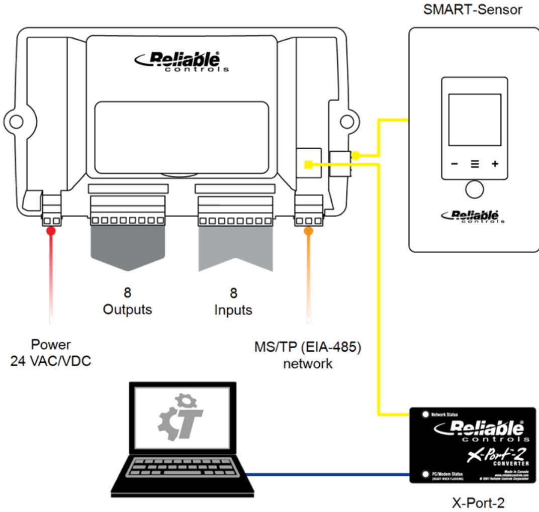
SMART-Net connection
